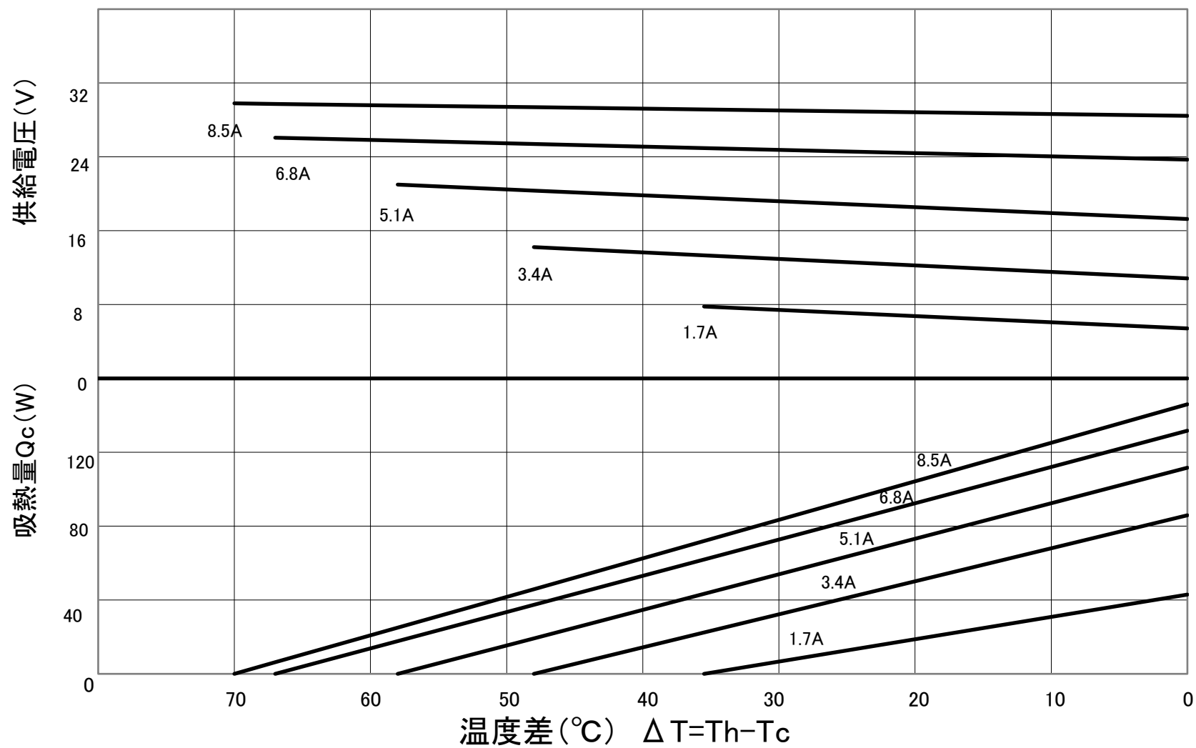
FPH1-24108BC特性図 (Th=27°C)
